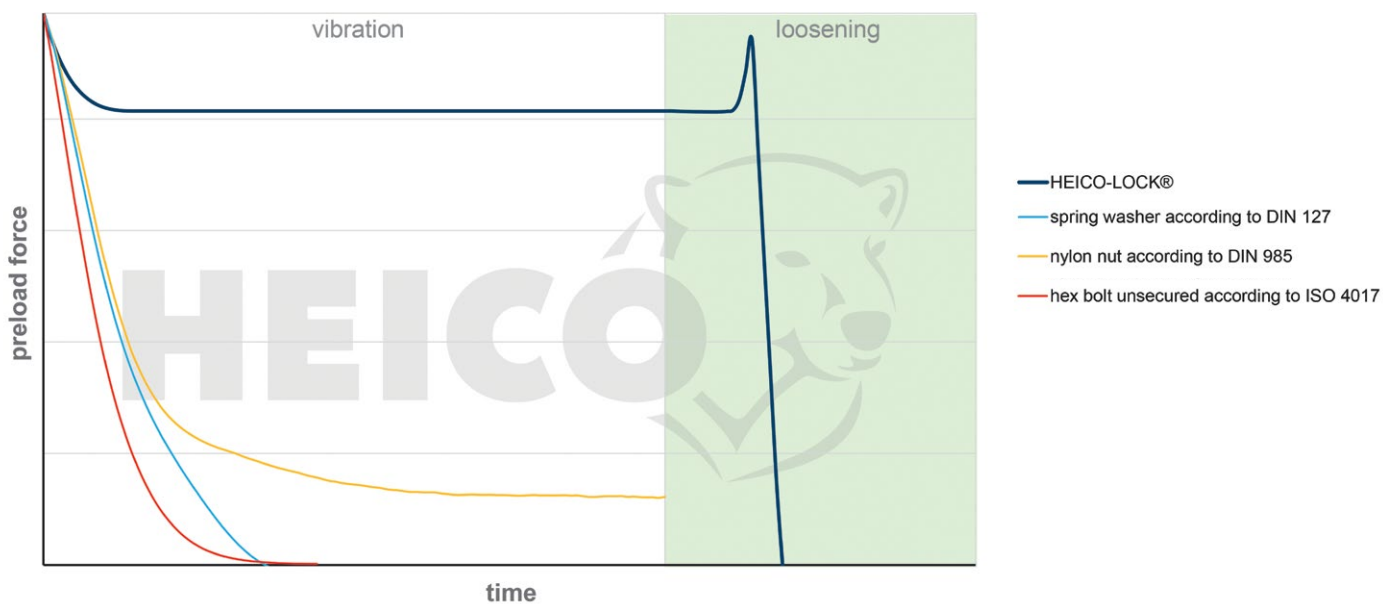
Chart: The process of preload force loss as demonstrated by vibration testing to DIN 65151 / DIN 25201-4
